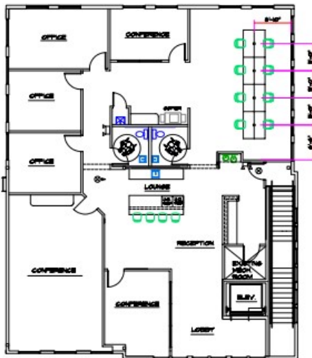
ELECTRICAL PLAN
